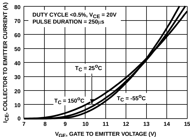
FIGURE 13. TRANSFER CHARACTERISTICS
