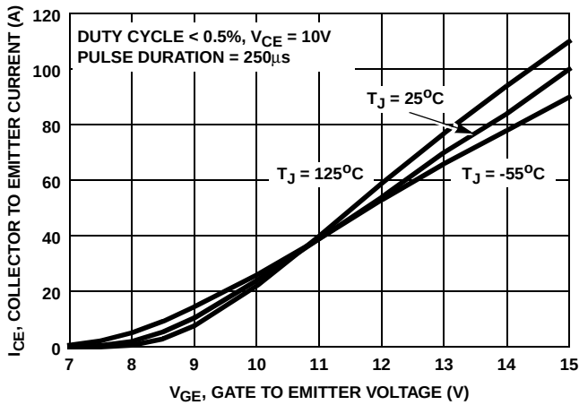
FIGURE 13. TRANSFER CHARACTERISTIC
