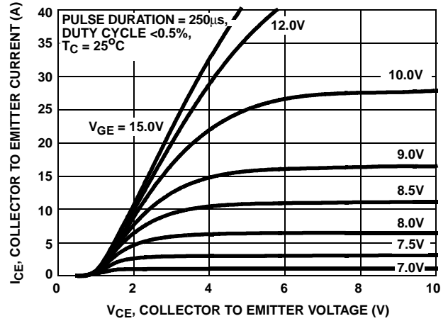
FIGURE 2. SATURATION CHARACTERISTICS
