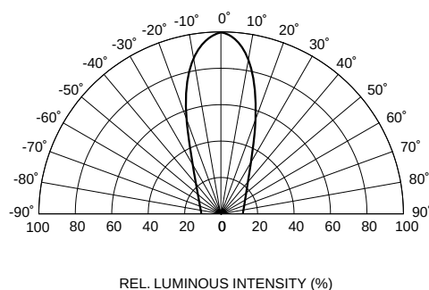
Fig. 5B Radiation Diagram (HLMP-K640)
