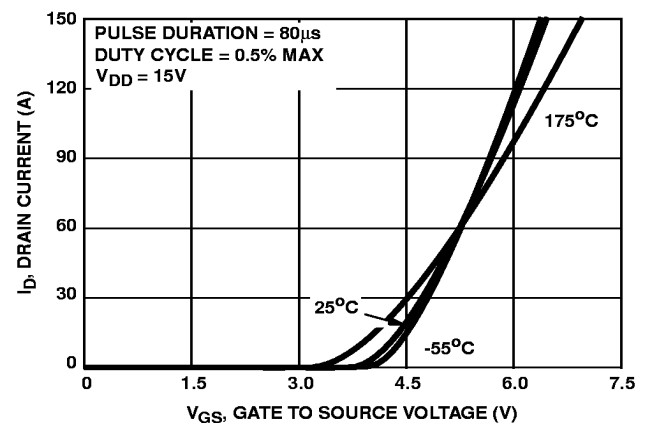
FIGURE 8. TRANSFER CHARACTERISTICS
