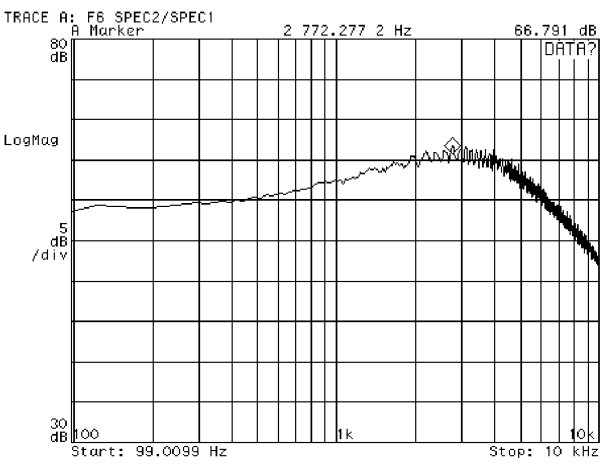
Ripple Rejection Load=80mA, C OUT =4.7μF
