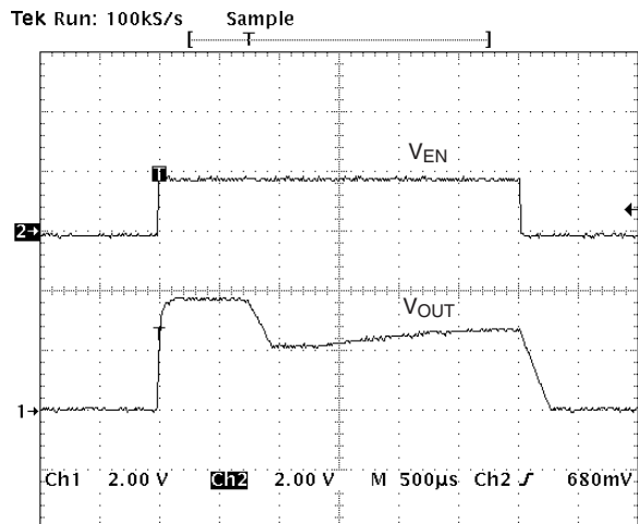
ON/OFF Transient Response Load=10mA, C_{OUT}=1\mu F C_N=10nF
