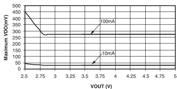
Dropout Voltage vs. Output Voltage
