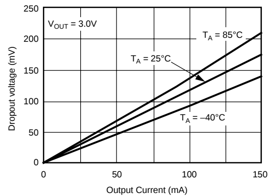
Dropout voltage vs I_{OUT}
