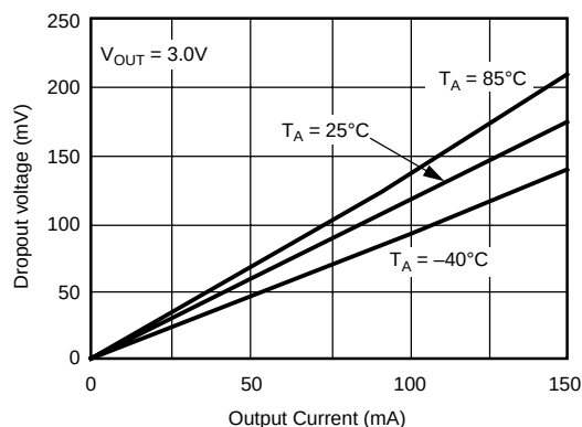
Dropout voltage vs I_{OUT}
