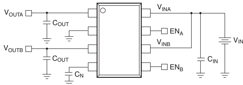
Figure 1. Test Circuit
