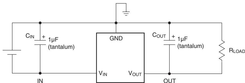
Figure 1. Test Circuit
