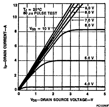
Figure 3 Output Characteristics
