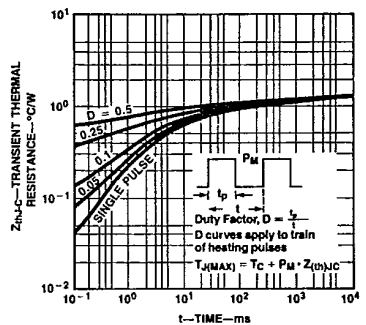
Figure 12 Transient Thermal Resistance vs Time for MTP12N18/12N20
