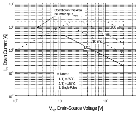
Figure 9-1. Maximum Safe Operating Area for IRF624B
