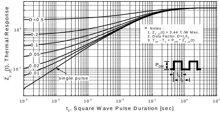
Figure 11-1. Transient Thermal Response Curve for IRF710B
