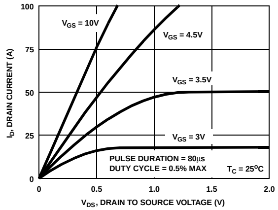
Figure 6. Saturation Characteristics
