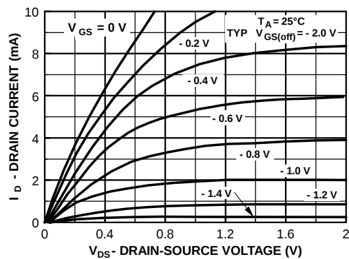
Common Drain-Source
