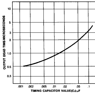
Figure 6. Output Stage Dead Time As A Function
