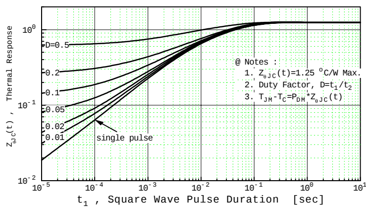
Figure 11. Thermal Response
