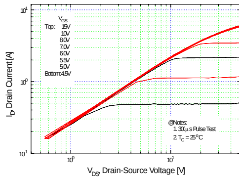
Figure 1. Output Characteristics
