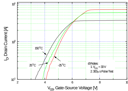
Figure 2. Thansfer Characteristics
