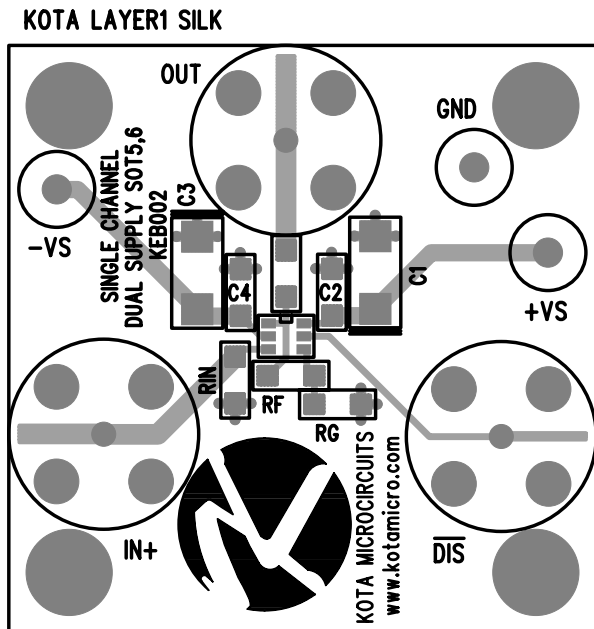
Figure 6a: KEB002 (top side)
