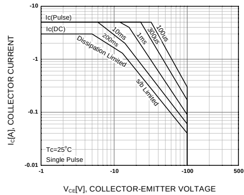
Figure 4. Forward Bias Safe Operating Area
