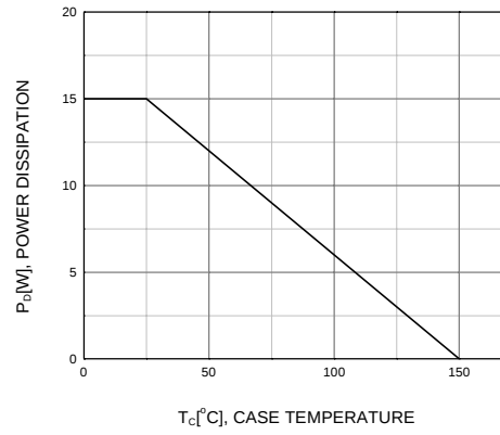
Figure 8. Power Derating
