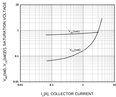
Figure 5. Base-Emitter Saturation Voltage Collect-Emmitter Saturation Voltage
