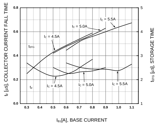
Figure 6. Switching Time
