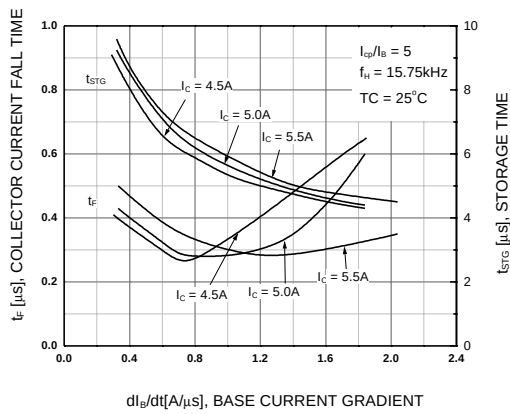
Figure 5. Switching Time
