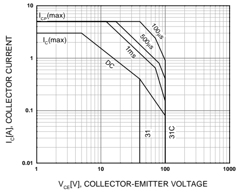
Figure 6. Safe Operating
