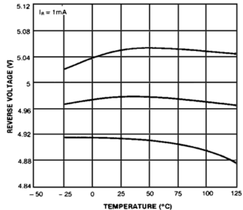
FIGURE 2. Reverse Characteristics
