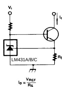
Figure 15. Constant-Current Sink
