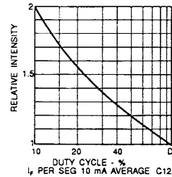
Fig. 4E. Relative Luminous Intensity vs. Duty Cycle
