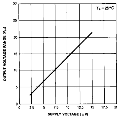
Figure 3. Output Swing
