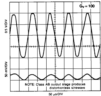
Figure 2. Wave Response
