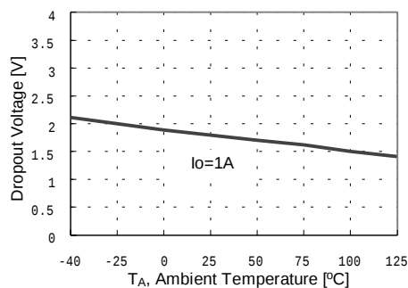
Figure 4. Dropout Voltage
