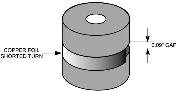
Figure 11. Copper Foil Shorted Turn
