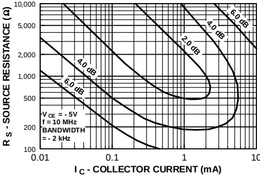
Contours of Constant Narrow Band Noise Figure
