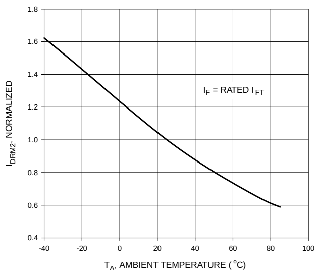
Figure 5. I_{\text{DRM2}} - Leakage in Inhibit State vs. Temperature
