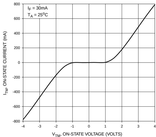
Figure 2. On-State Characteristics
