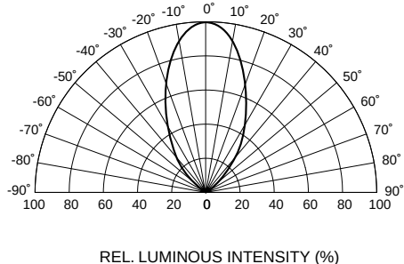
Fig. 3 Radiation Diagram
