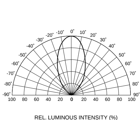
Fig. 3 Radiation Diagram
