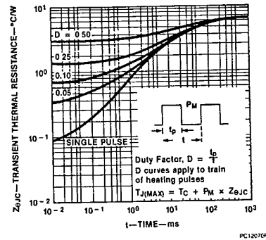
Figure 10 Transient Thermal Resistance vs Time for IRF510-513
