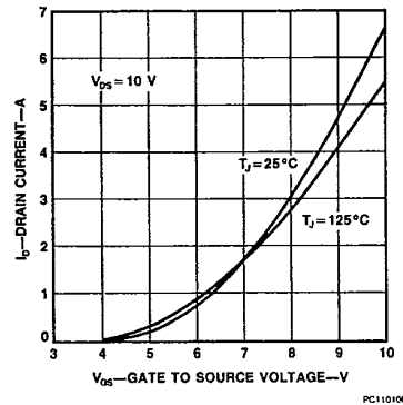
Figure 3 Transfer Characteristics
