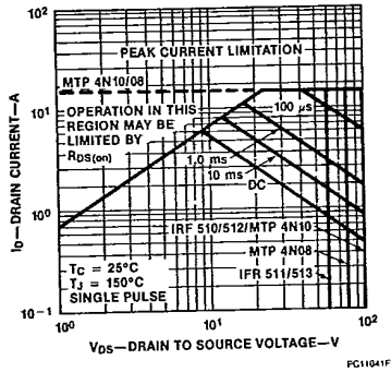
Figure 9 Forward Biased Safe Operating Area for IRF510-513
