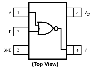
Pad Assignments for MicroPak
