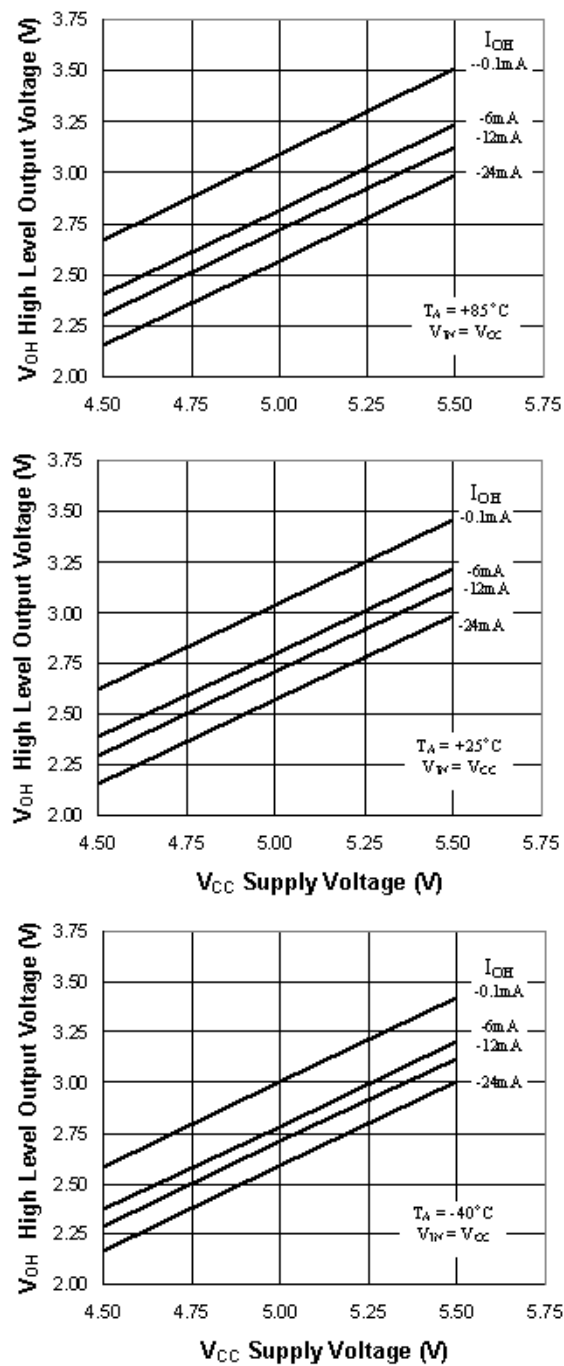
FIGURE 3. Typical High Level Output Voltage vs. Supply Voltage
