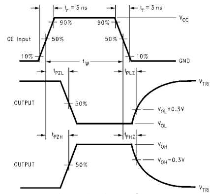
FIGURE 3. AC Waveforms
