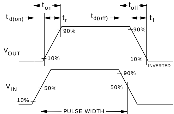
Figure 12. Switching Waveforms.
