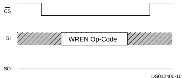
FIGURE 8. Write Enable
