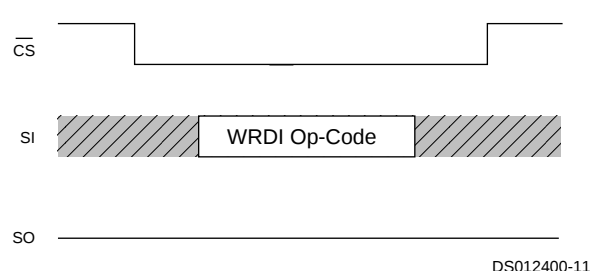
FIGURE 9. Write Disable
