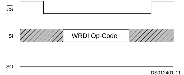
FIGURE 9. Write Disable
