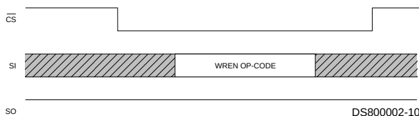
FIGURE 7. Write Enable
