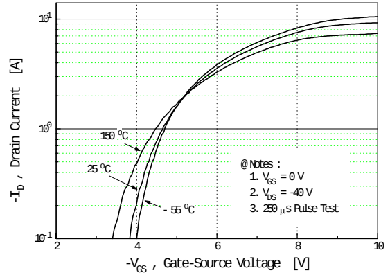
Fig 2. Transfer Characteristics
