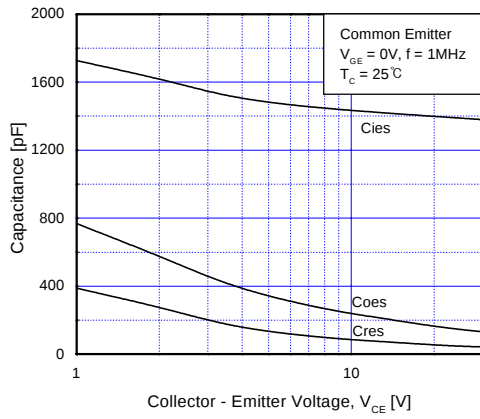
Fig 7. Capacitance Characteristics
