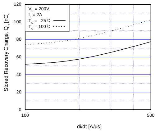
Fig 20. Stored Charge
