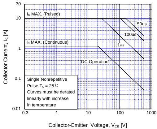
Fig 15. SOA Characteristics
