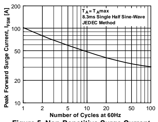
Figure 5. Non-Repetitive Surge Current
