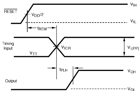
FIGURE 7. Voltage Waveforms - RESET Removal Delay Times
