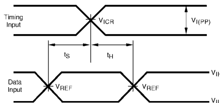
FIGURE 5. Voltage Waveforms - Setup and Hold Times
