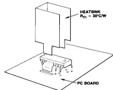
EXAMPLE OF CIRCUIT WITH EXTERNAL HEATSINK
